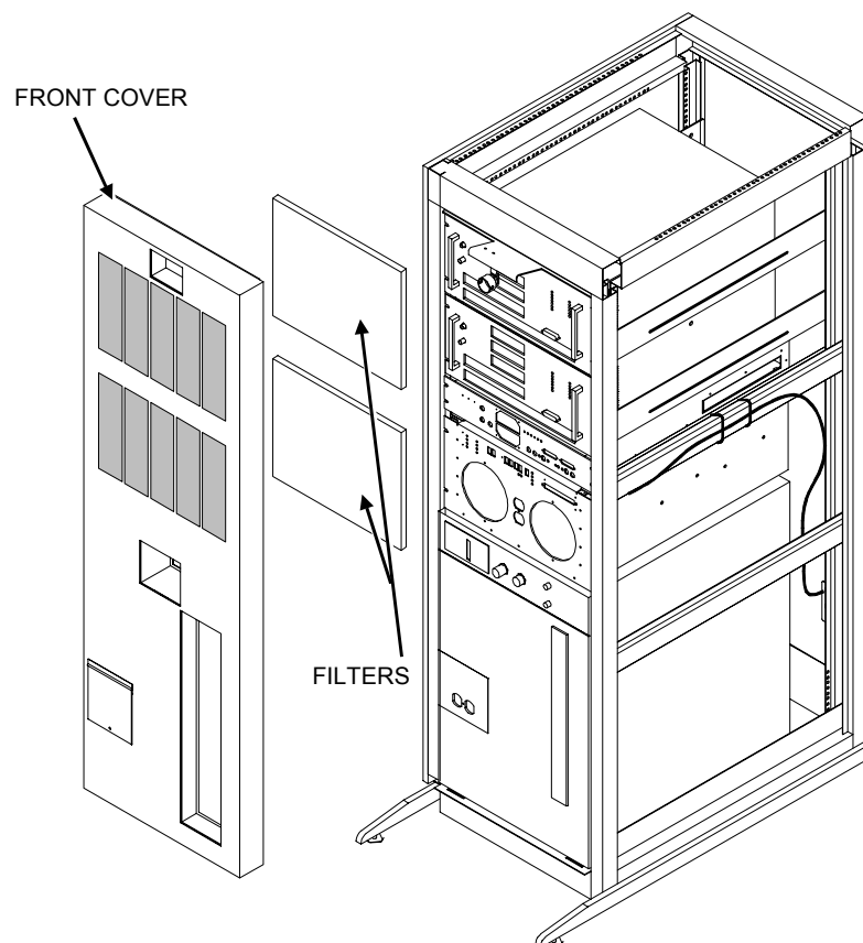
RF/PDU CABINET COVER AND FILTER LOCATIONS ILLUSTRATION 2-1
