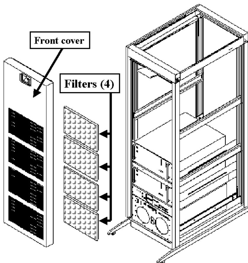
SRF CABINET COVER AND FILTER LOCATIONS ILLUSTRATION 2-2
